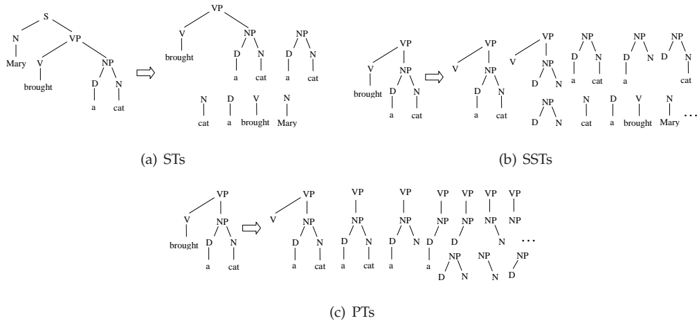
Figure 1 Example of ST (a), SST (b) and PT (c) fragments.
