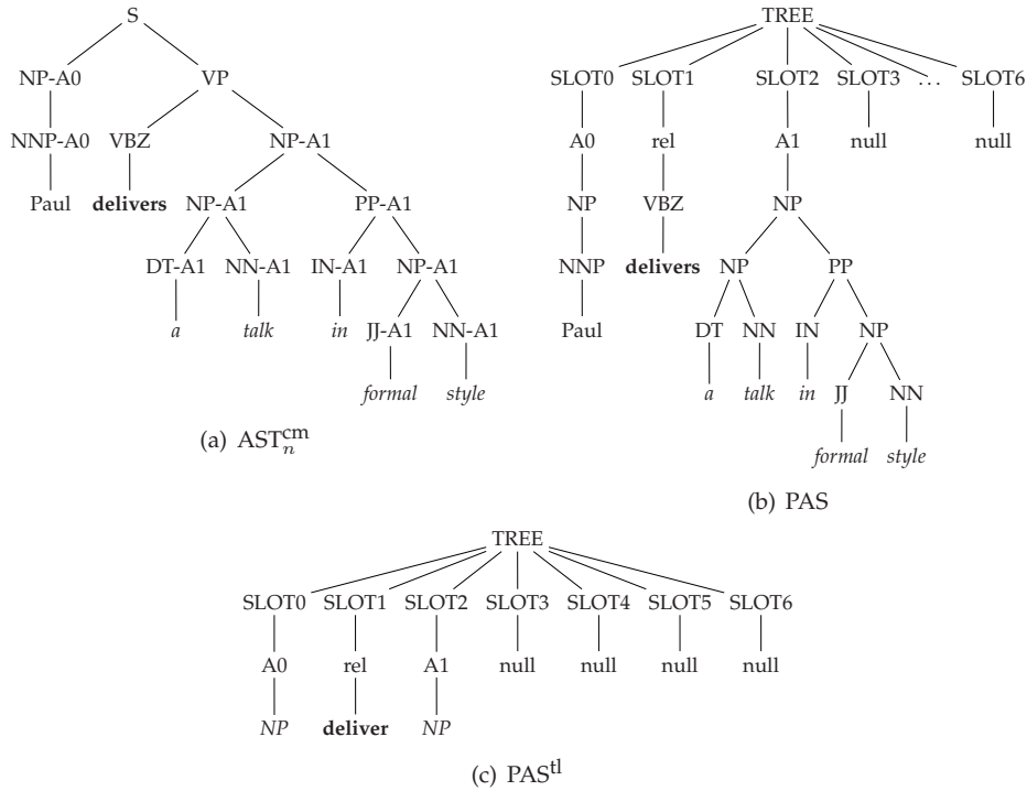
Figure 8 Different representations of a same proposition.
